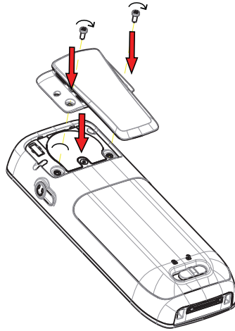
Figure 18. Screw the hinge-type clip into position.
